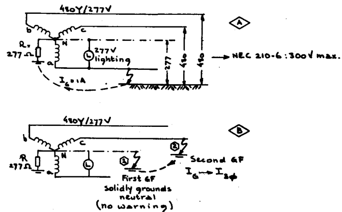
Fig. 9. Illustration showing why three-phase, four-wire (480 wye/277V) systems cannot be resistance grounded.
