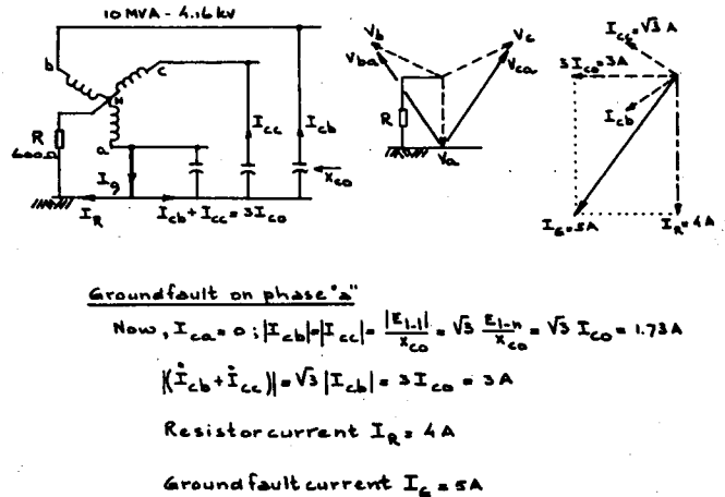
Fig. 2. Voltage and current relationship in high-resistance neutral grounded system during a ground fault on phase "a".
