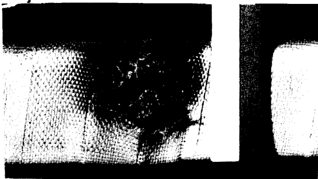
Fig. 8. Resulting burning damage due to simulated 3A, 16 minute ground-fault test.
