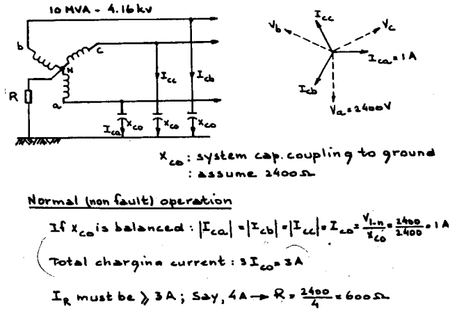
Fig. 1. Voltage and charging current relationship in high-resistance neutral grounded system during normal operation.
