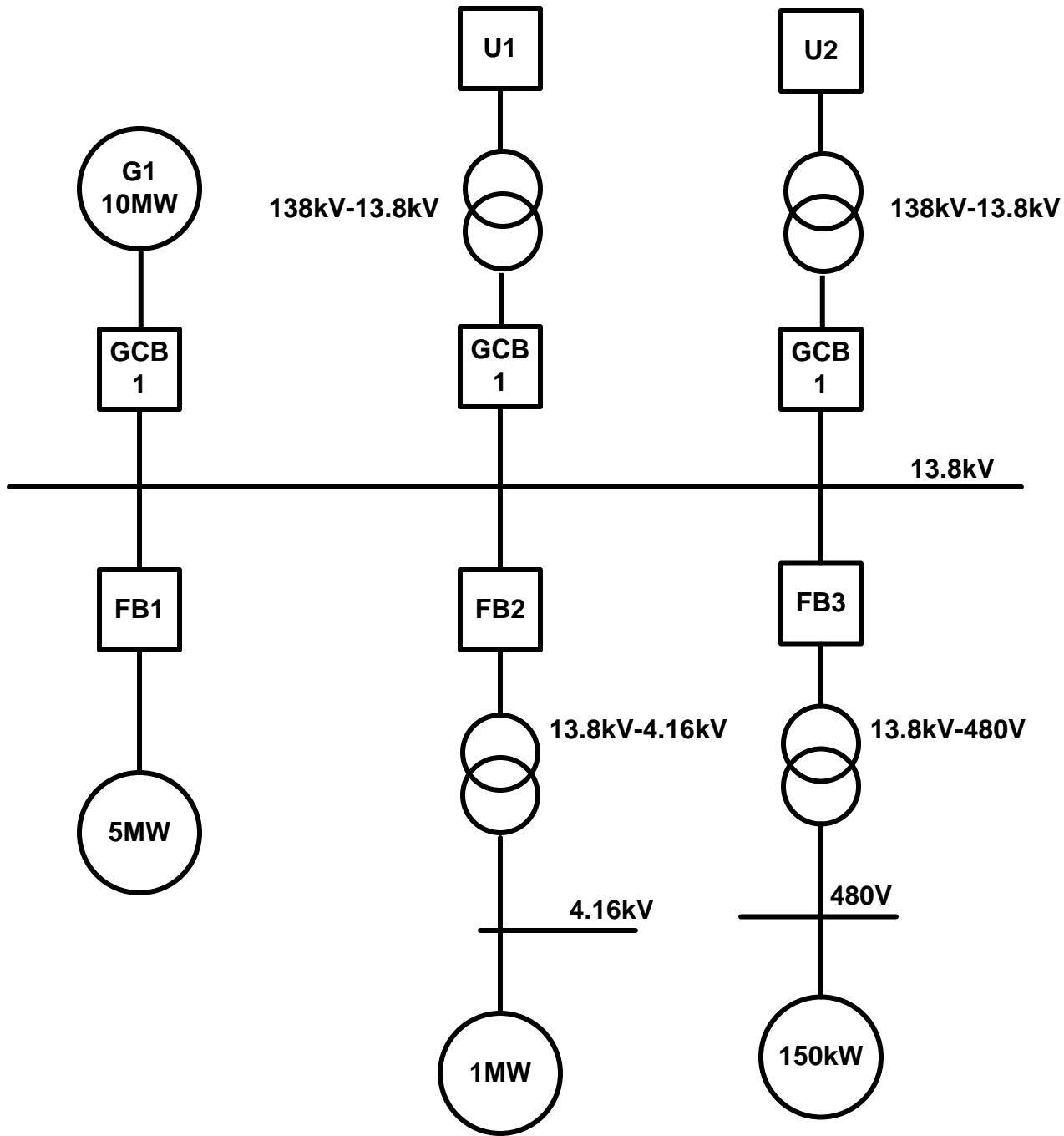
EXAMPLE PLANT COGEN
