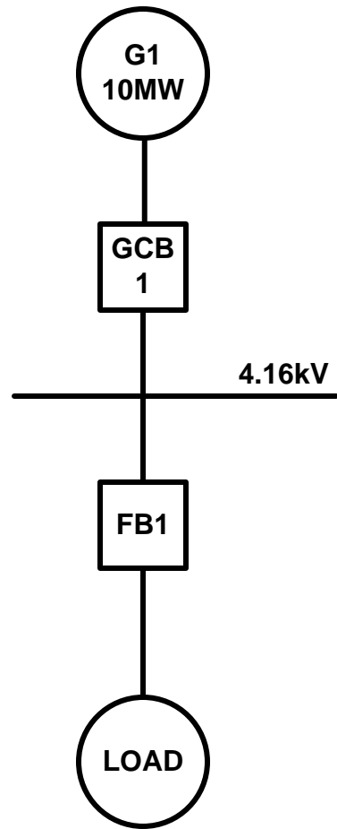
EXAMPLE ISLAND BUS CONNECTED / 1 GTG
