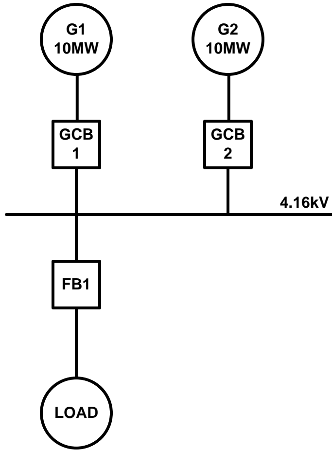
EXAMPLE ISLAND BUS CONNECTED / 2 GTG
