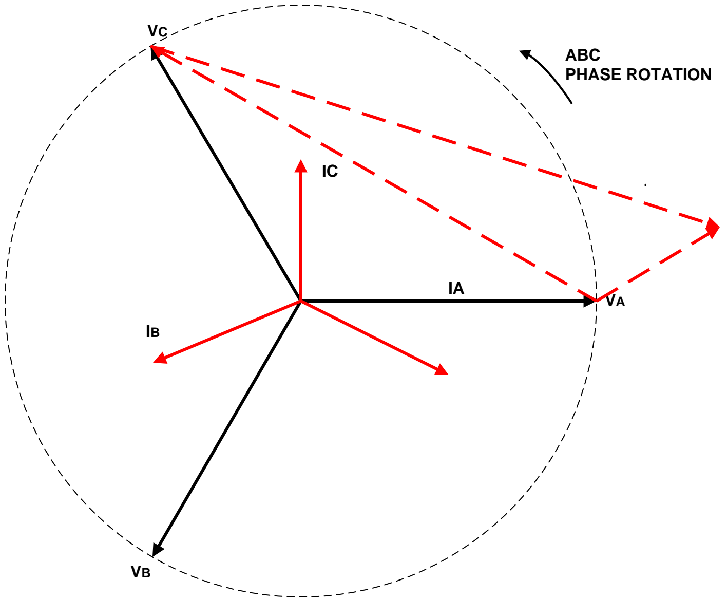
3-PHASE A-B-C Rotation with Lagging Load but I_b polarity into AVR is reversed
